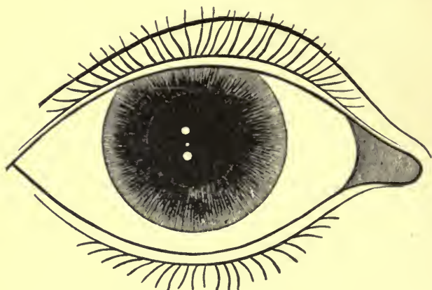
FIG. 59.—Reflections from same two lights when the lens is in alignment, (Tscherning).
